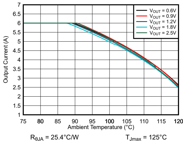
Figure 8-40. Safe Operating Area V_{IN} = 3.3\text{-V} TPSM82866AA0HRDMR
