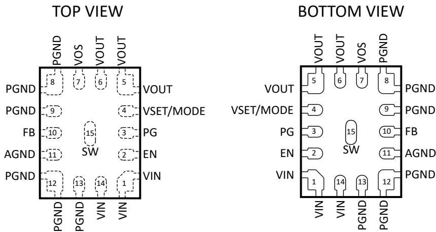
Figure 5-1. TPSM82864A, TPSM82866A - RCF (15 Pin) QFN-FCMOD
