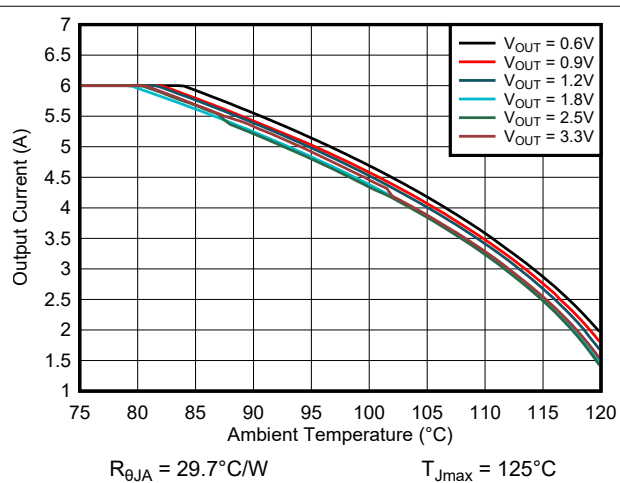
R_{\theta JA} = 29.7^\circ\text{C/W} T_{Jmax} = 125^\circ\text{C} Figure 8-37. Safe Operating Area V_{IN} = 5.0\text{ V} TPSM82866AA0PRCFR
