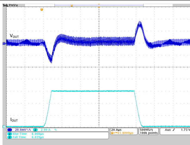
V_{IN} = 5.0\text{ V} V_{OUT} = 1.2\text{ V} T_A = 25^\circ\text{C}
