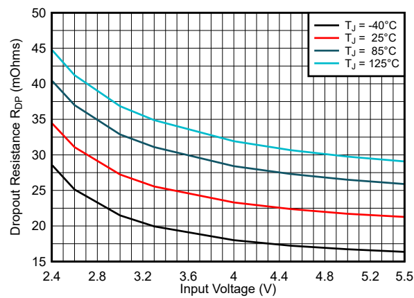
Figure 6-5. Dropout Resistance R DP
