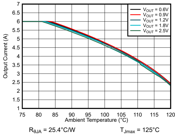
Figure 8-38. Safe Operating Area V_{IN} = 3.3\text{-V} TPSM82866AA0SRDJR
