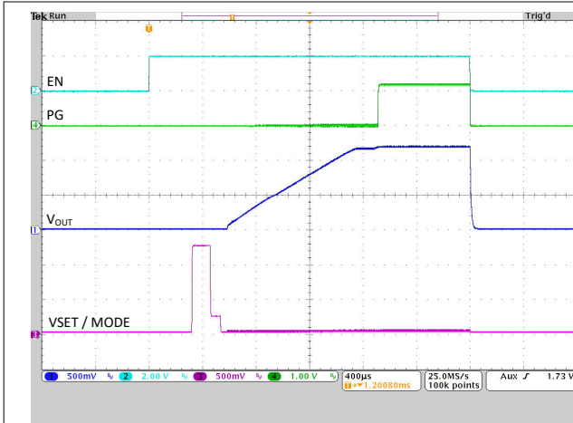
R_{VSET} = 56.2\text{ k}\Omega I_{OUT} = 6.0\text{ A} Figure 8-32. Start-Up into Full Load
