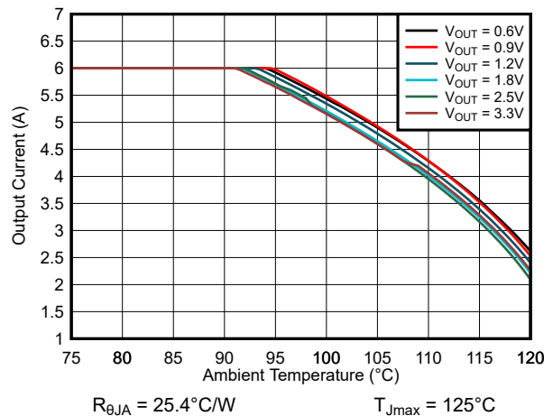
Figure 8-41. Safe Operating Area V_{IN} = 5.0\text{-V} TPSM82866AA0HRDMR
