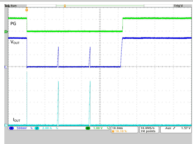
R_{LOAD} = 100\text{ m}\Omega (during overload) Figure 8-35. HICCUP Short-Circuit Protection
