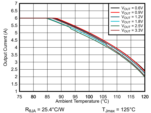
Figure 8-39. Safe Operating Area V_{IN} = 5.0\text{-V} TPSM82866AA0SRDJR
