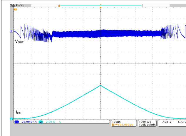
V_{IN} = 5.0\text{ V} V_{OUT} = 1.2\text{ V} T_A = 25^\circ\text{C} Figure 8-34. Load Sweep I_{OUT} = 20\text{ mA} \rightarrow 6\text{ A}
