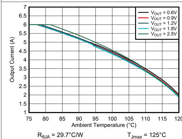
R_{\theta JA} = 29.7^\circ\text{C/W} T_{Jmax} = 125^\circ\text{C} Figure 8-36. Safe Operating Area V_{IN} = 3.3\text{ V} TPSM82866AA0PRCFR
